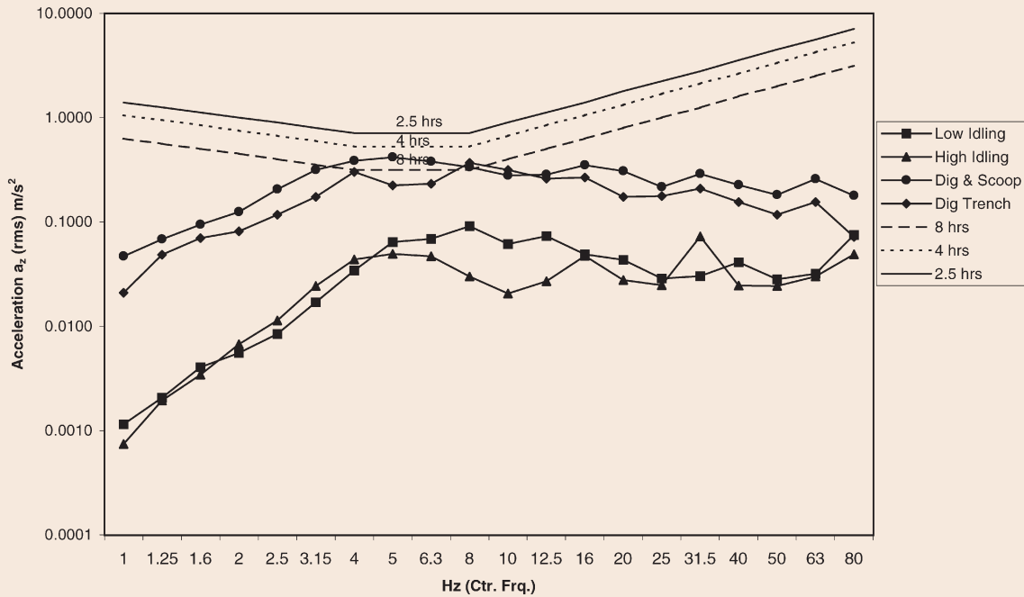
*Whole-body vibration from a medium-size excavator (OE #4) in the longitudinal (Z-axis) compared to the ISO/TLV limit.
