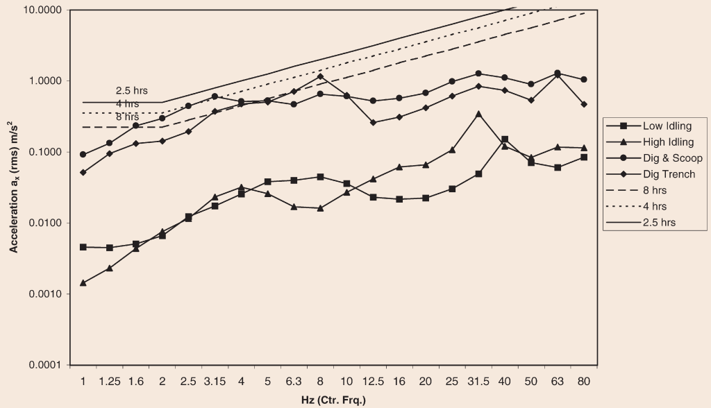
*Whole-body vibration from a medium-size excavator (OE #4) in the transverse (X-axis) compared to the ISO/TLV limit.
