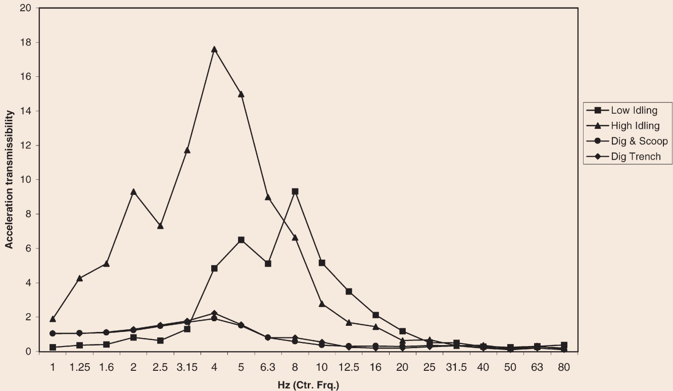
*Acceleration transmissibility for a medium size excavator (OE #4) in the longitudinal (Z-axis).
