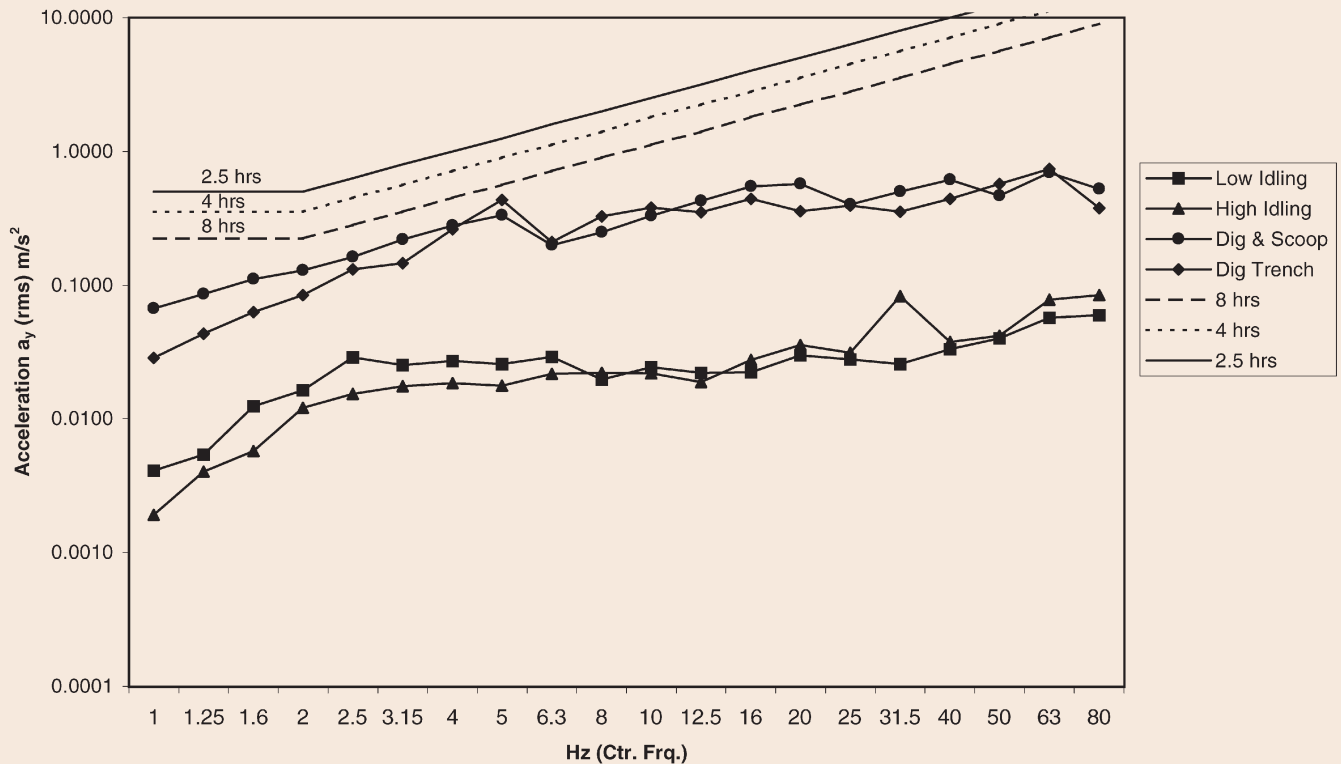
*Whole-body vibration from a medium-size excavator (OE #4) in the transverse (Y-axis) compared to the ISO/TLV limit.
